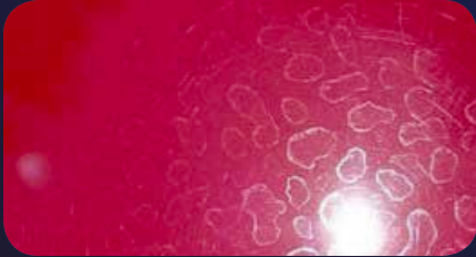
Acid Rain
